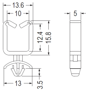
CHASSIS Ø5.0 THICKNESS 0.8~1.6
