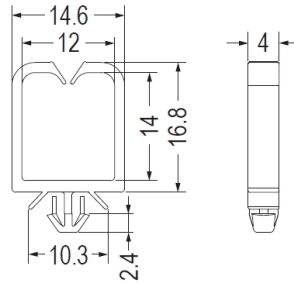
CHASSIS Ø4.0 THICKNESS 0.8-2.0
