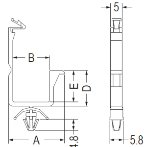
CHASSIS Ø4.8 THICKNESS 2.0~3.0
