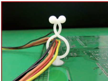
MOUNTING HOLE Ø4.8~Ø5.0 THICKNESS 1.2~2.0
