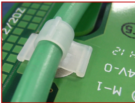
CHASSIS \varnothing 6.0\text{--}\varnothing 6.5 THICKNESS 0.8~2.5
