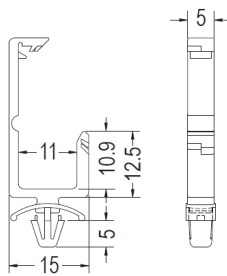
CHASSIS Ø4.8 THICKNESS 0.8-2.0
