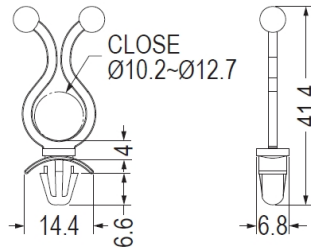
CHASSIS Ø6.0 THICKNESS 0.78~2.0
