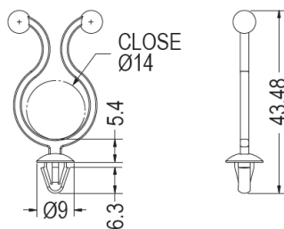
MOUNTING HOLE Ø4.8~Ø5.0 THICKNESS 1.2~2.0
