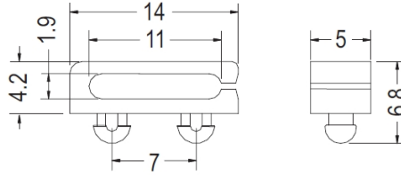
MOUNTING HOLE \varnothing 3.0 THICKNESS 0.8~1.0
