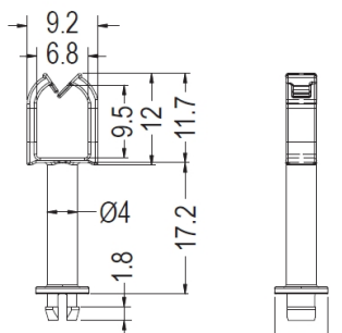
CHASSIS Ø3.8 THICKNESS 1.7
