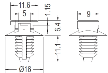
MOUNTING HOLE Ø6.4~Ø7.1 THICKNESS 0.8~6.0
