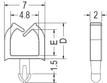
MOUNTING HOLE Ø1.7 THICKNESS: T
