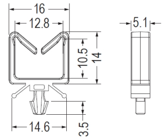
CHASSIS Ø3.4~Ø3.5 THICKNESS 2.5
