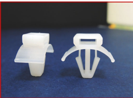
MOUNTING HOLE Ø6.2~Ø6.3 THICKNESS 0.8~3.6
