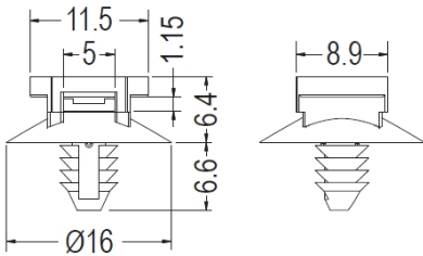
MOUNTING HOLE Ø4.5~Ø5.0 THICKNESS 0.8~7.0
