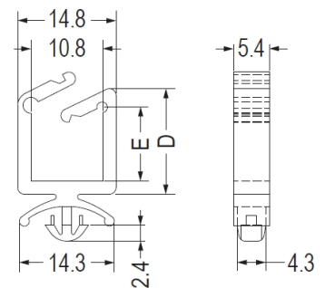
CHASSIS Ø4.8 THICKNESS 0.8-1.6
