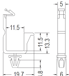
CHASSIS Ø4.8 THICKNESS 1.6
