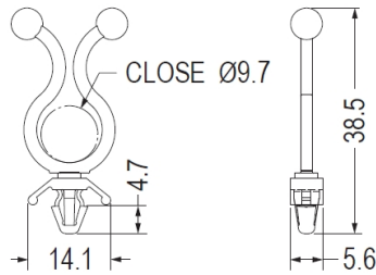
CHASSIS Ø4.8 THICKNESS 0.8~2.5
