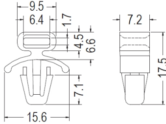
MOUNTING HOLE Ø6.4 THICKNESS 1.2-2.8
