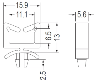
CHASSIS: ØG THICKNESS 0.8~1.6
