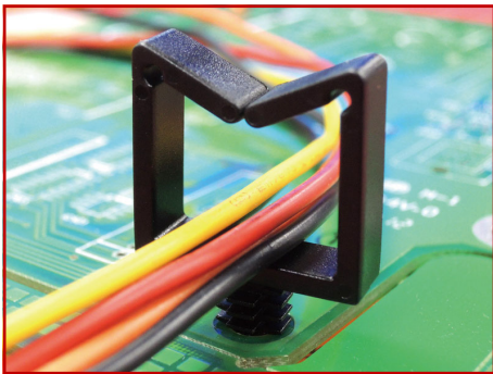
CHASSIS Ø5.3
