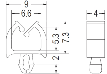
P.C.B Ø3.0 THICKNESS 1.2~1.6
