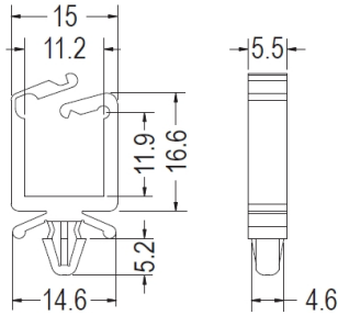
CHASSIS Ø4.8 THICKNESS 0.8-1.8
