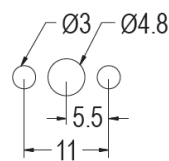
MOUNTING HOLE THICKNESS 0.5~1.6
