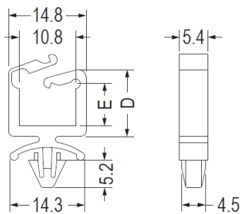
CHASSIS Ø4.8-Ø5.0 THICKNESS 0.5-2.0
