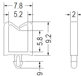
MOUNTING HOLE Ø2.0 THICKNESS: T
