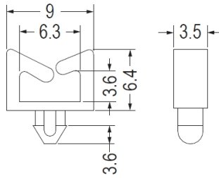
CHASSIS Ø3.0 THICKNESS 1.2~1.6
