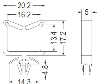
CHASSIS Ø4.8 THICKNESS 1.0~2.5
