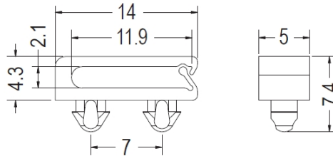
MOUNTING HOLE \varnothing 3.0 THICKNESS 0.8~1.0
