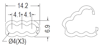
UNIT FOLDED VIEW
