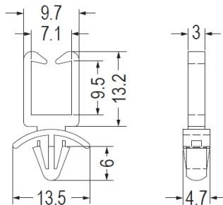
CHASSIS Ø4.8 THICKNESS 0.8~1.6
