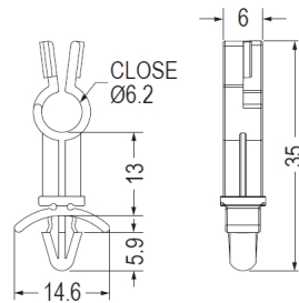
CHASSIS Ø4.8-Ø5.0 THICKNESS 0.7-2.0
