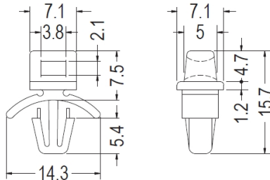
MOUNTING HOLE Ø4.8 THICKNESS 0.8~2.0
