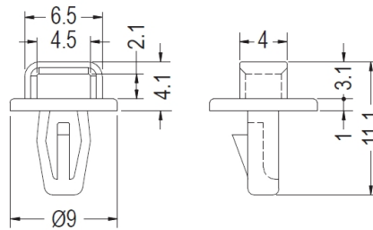
MOUNTING HOLE Ø4.0 THICKNESS 1.6~2.0
