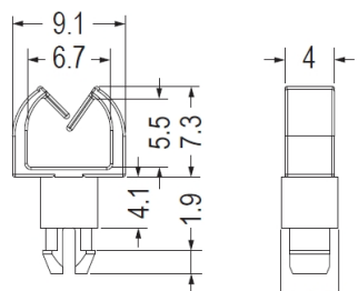
CHASSIS Ø3.8 THICKNESS 1.6
