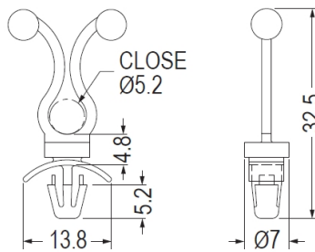
CHASSIS Ø4.8 THICKNESS 0.8~2.0
