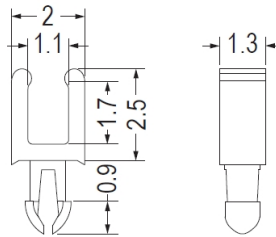
MOUNTING HOLE Ø1.0 THICKNESS 1.0
