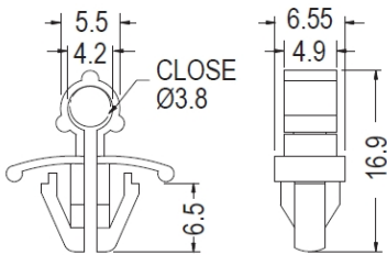
CHASSIS \varnothing 6.5 THICKNESS 1.2
