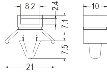
MOUNTING HOLE Ø6.2 THICKNESS 0.8-3.2
