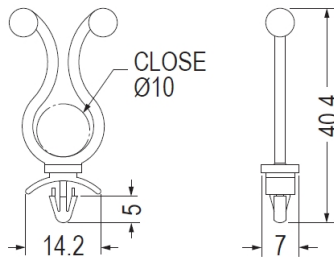
CHASSIS Ø4.0 THICKNESS 0.8~2.0
