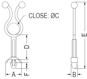
CHASSIS: ØG THICKNESS 0.8~2.2
