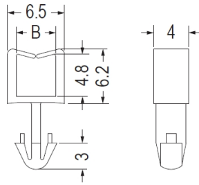
CHASSIS Ø3.5 THICKNESS: T
