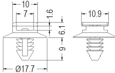
MOUNTING HOLE Ø6.0 THICKNESS 0.8~9.0
