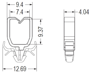
CHASSIS Ø3.5 THICKNESS 0.6-1.6
