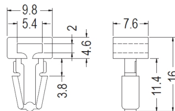
PANEL HOLE DIA Ø6.4 PANEL THICKNESS 3.17
