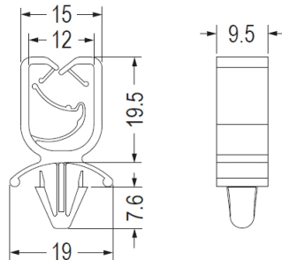
CHASSIS Ø6.3-Ø7.0 THICKNESS 0.6-3.0
