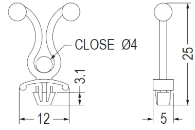
CHASSIS Ø4.0 THICKNESS 0.8~2.0
