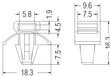
MOUNTING HOLE Ø6.2~Ø6.3 THICKNESS 0.8~3.6
