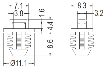
CHASSIS Ø7.9 THICKNESS 6.4
