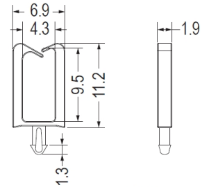
CHASSIS Ø1.75 THICKNESS 2.2
