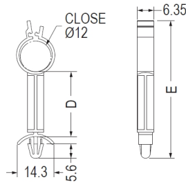
CHASSIS Ø4.8 THICKNESS 0.8-2.0
