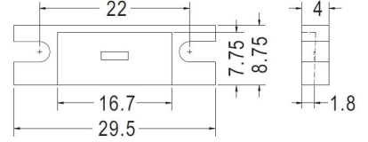
MOUNTING HOLE
