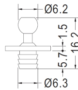
PIN CHASSIS Ø6.1 THICKNESS 6.4
