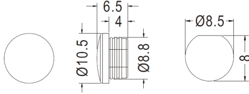
MOUNTING HOLE
