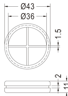
MOUNTING HOLE Ø40.0 THICKNESS 2.0
