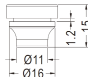
MOUNTING HOLE Ø11.5 THICKNESS 1.2~1.5
