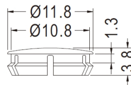
MOUNTING HOLE Ø11.0
