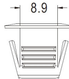
MOUNTING HOLE Ø12.0 CHASSIS THICKNESS 3.0
