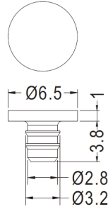
MOUNTING HOLE Ø3.0
