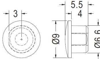
MOUNTING HOLE Ø6.35
