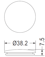
MOUNTING HOLE Ø31.5 THICKNESS 1.6
