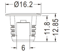
MOUNTING HOLE Ø12.0 CHASSIS THICKNESS 3.0
