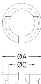
MOUNTING HOLE: ØG THICKNESS: T
