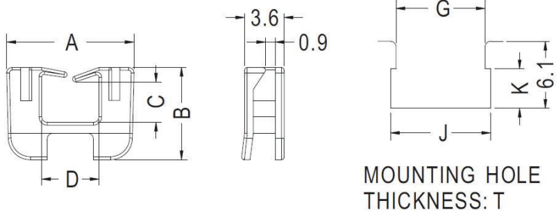
MOUNTING HOLE THICKNESS 1.2
