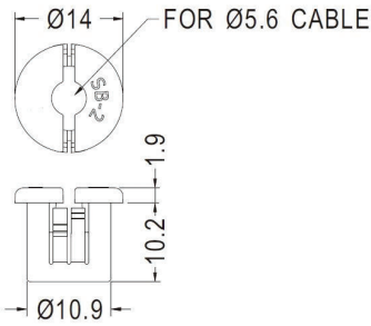
MOUNTING HOLE Ø11.1 THICKNESS 0.6~3.2
