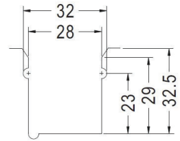
MOUNTING HOLE THICKNESS 3.0
