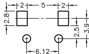
MOUNTING HOLES
