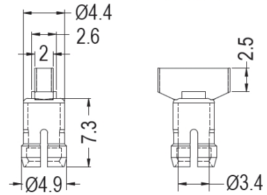
MOUNTING HOLE
